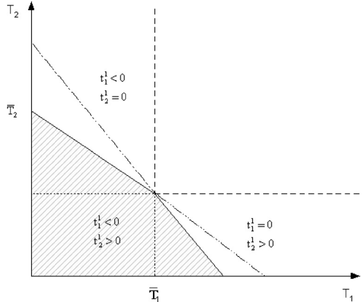
Fig. 2. The trading region if \Delta_1 \sigma_1^2 / \sigma_{12} > -\Delta_2 > \Delta_1 \sigma_{12} / \sigma_2^2 > 0 .
