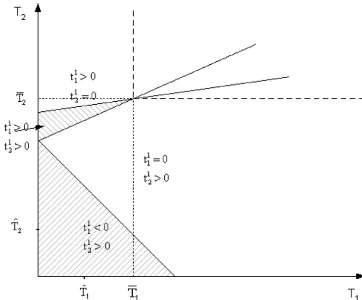
Fig. 1. The trading region if 0 < \Delta_1 \sigma_1^2 / \sigma_{12} < -\Delta_2 .
