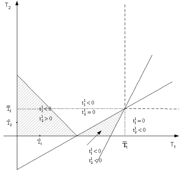
Fig. 3. The trading region if 0 < -\Delta_2 < \Delta_1 \sigma_{12} / \sigma_2^2 .
